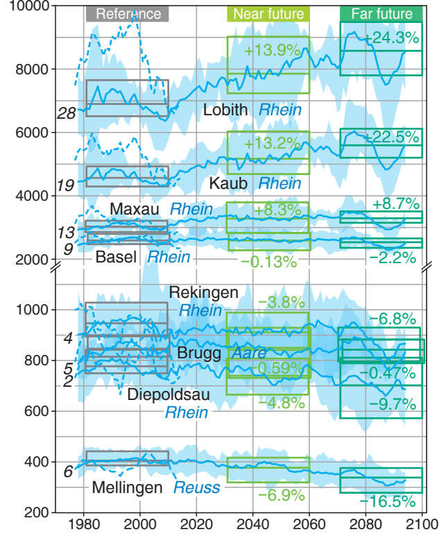
Figure 18: Time series of modeled high flows (annual 1-day maxima, HQ) and low flows (annual 7-day-minima, AM7) at gauging stations in the Rhine basin (11-year moving averages).
