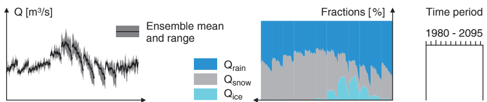
Figure 16: Time series of modeled streamflow and the percentages of its components Q_{rain} , Q_{snow} , and Q_{ice} for each month and year (11-year moving averages from 1980–2095). The component fractions (right axis) represent ensemble means.
